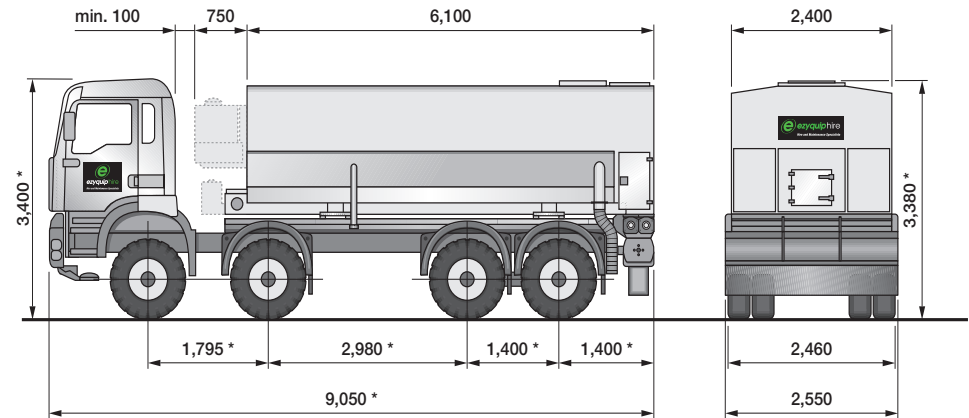
Binding agent spreader SW 20 MC Built-up unit with 4-axle truck Dimensions in mm
